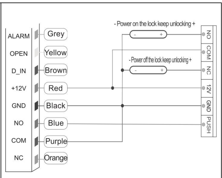
Fig. 2 Special power supply diagram
